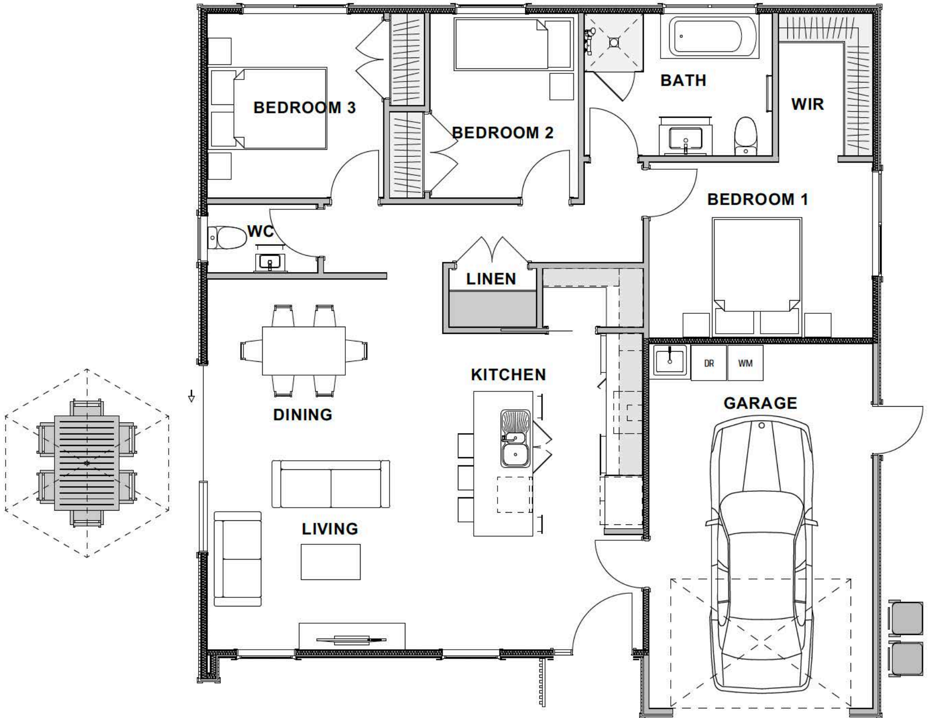
STAGE 3A FLOOR PLAN
